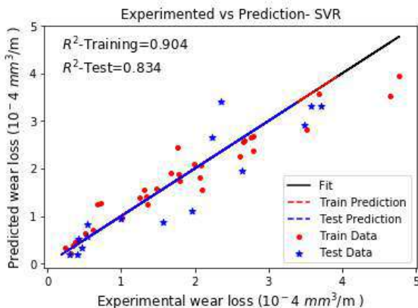
Fig 2. Wear loss prediction using SVR
