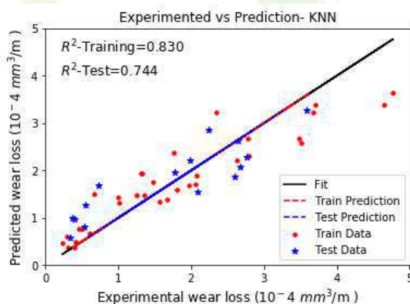
Fig 1. Wear loss prediction using KNN
